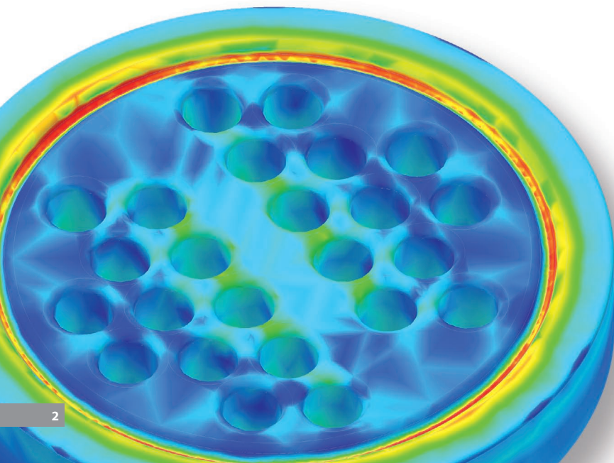
Finite Element Analysis (FEM) for determining the stress on the tube base in order to improve the operational reliability
