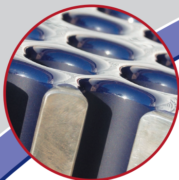
Cross-sectional view of a glass lined tubesheet note the machined glass inside. The gasket-free tube/tubesheet connection guarantees perfect fitting
