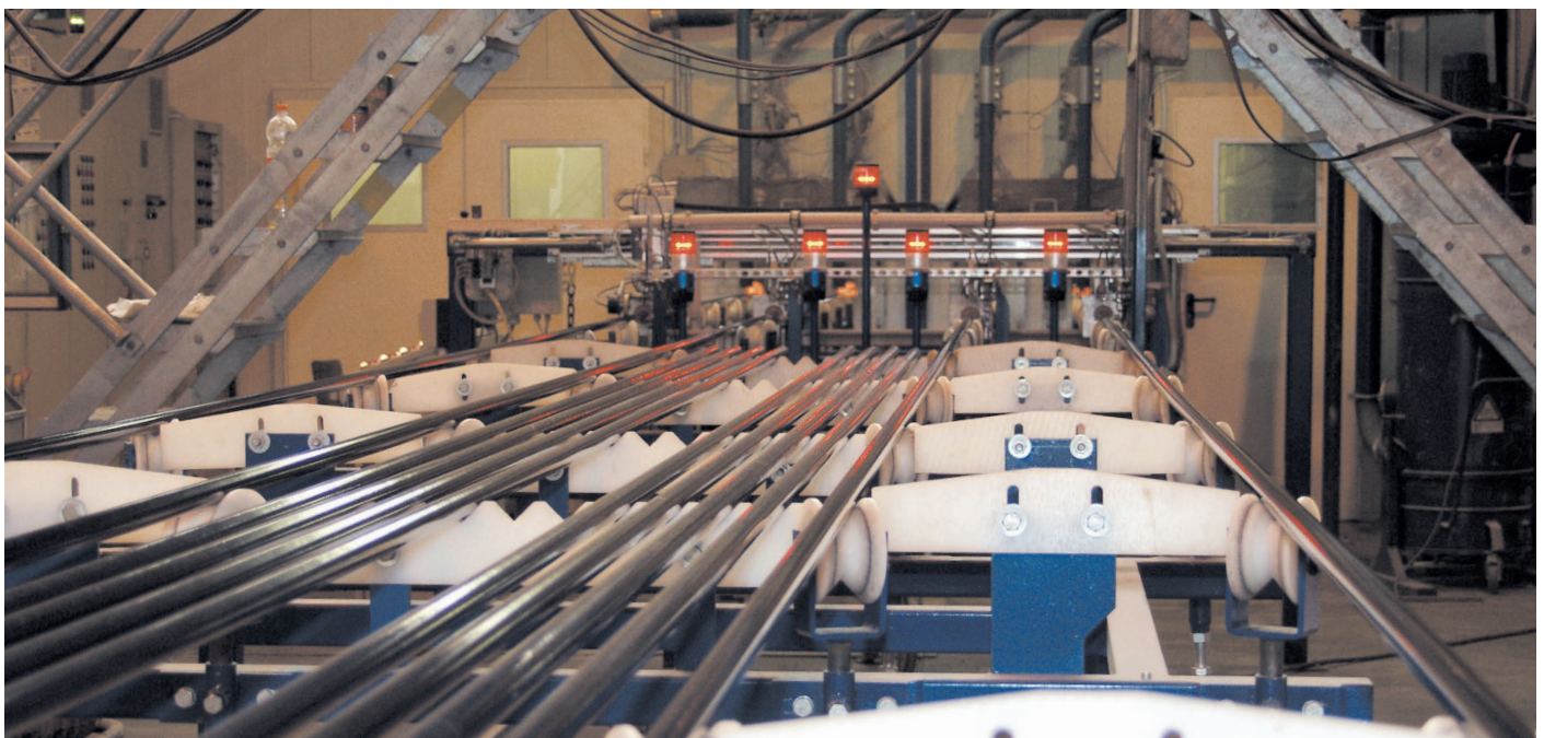
Fully automatic production line for manufacturing glass lined tubes using the dry electrostatic coating method
